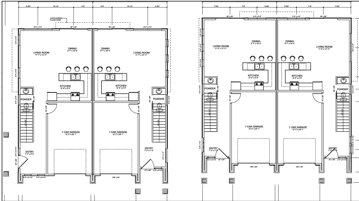
Figure 11 - Main Level Floor Plan
