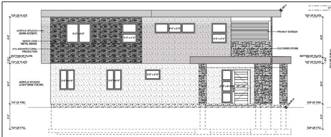
Figure 13 - Front Elevation (Facing East to Government Street)
