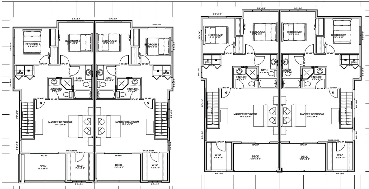
Figure 12 - Second Level Floor Plan
